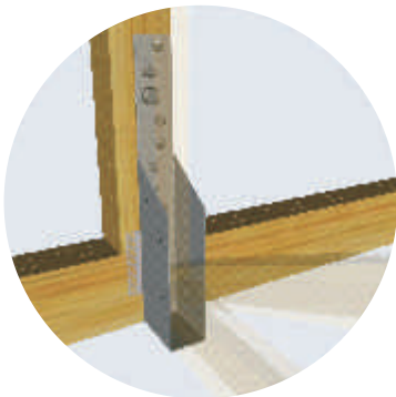
Principal truss shoe supporting primary hip girder
