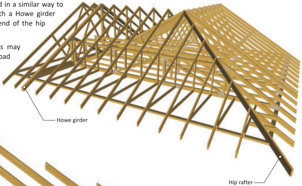
Hip rafter
