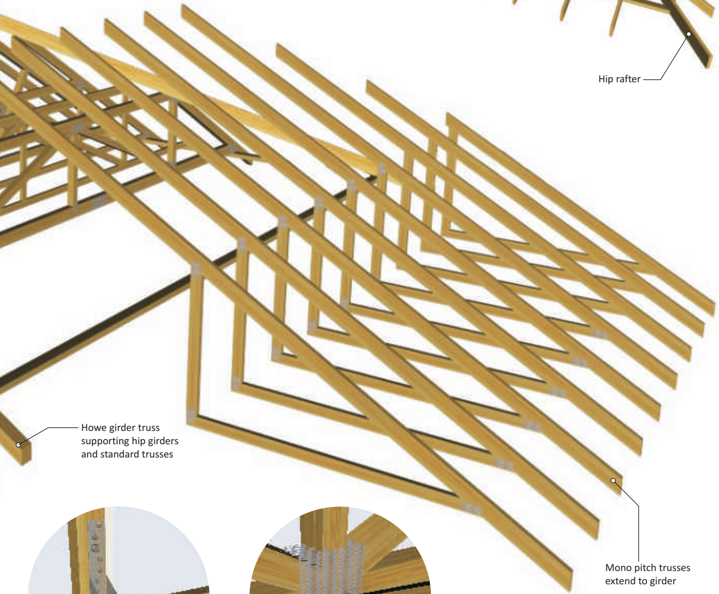
Howe girder
